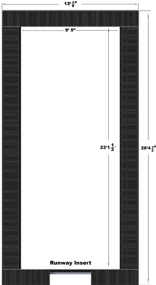
UCS Pour-in-Place Long Jump Pit Form System A Modular Perfect Fit System
